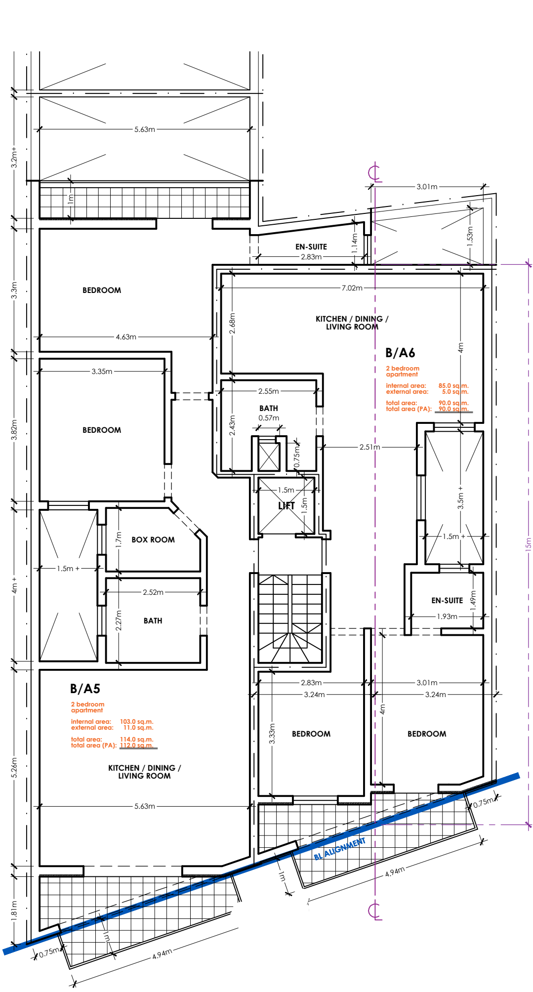
PROPOSED - CLEAN COPY Third floor level scale 1:100 .
